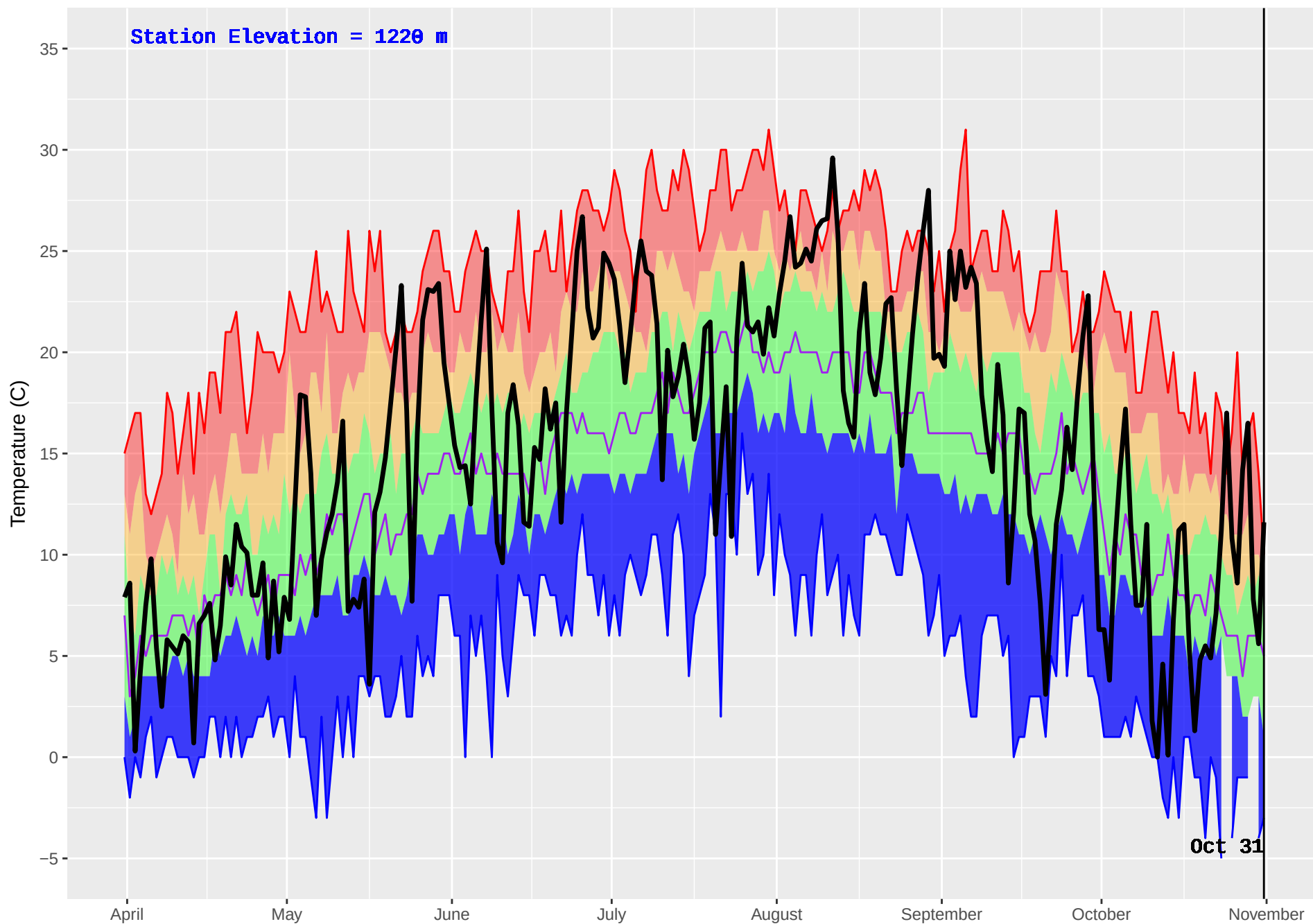
NEMIAH (216) : Historical (1982–2016) and Current (2017) Noon Temperature
